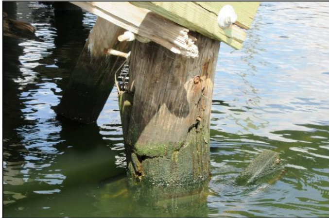
Timber pile broken at waterline
